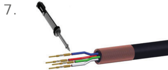
Crimp or solder one contact (1) each on every conductor ⚠ Tin-solder must not remain on contact surface!
