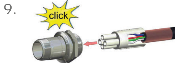
Put insulation part (2) into housing (3) 🗨 Pay attention to notches.
